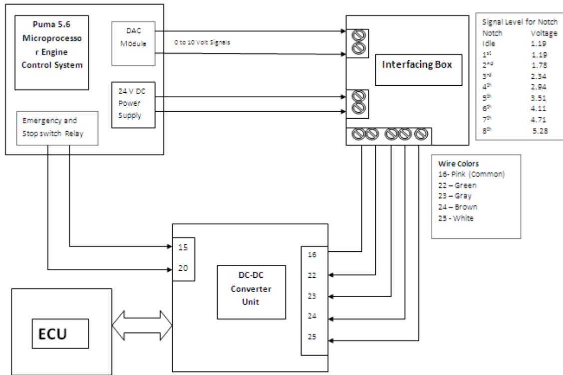
Figure: Block Diagram of Interfacing Box to PUMA 5.6
