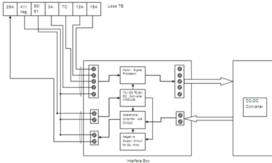
Figure: Block Diagram of Interfacing Box between MBCS and EFI ECU
