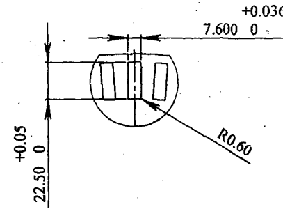
DETAIL H SCALE 1 : 2
