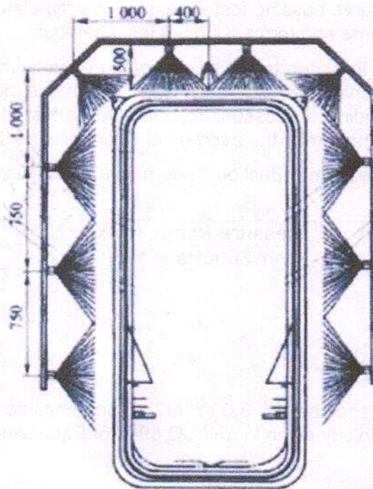
Fig.1 : Spray arrangements of Gangway
