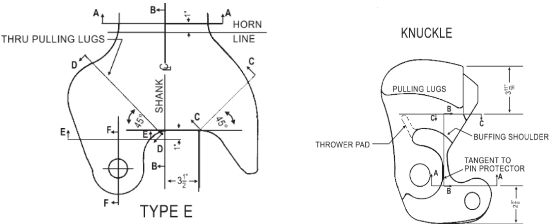
Coupler Head
