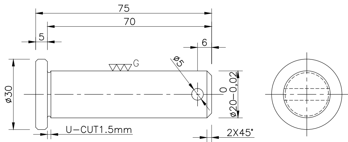
PIN-01 NO
