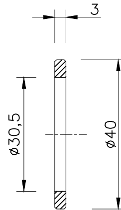
MACHINED WASHER-01 NO
