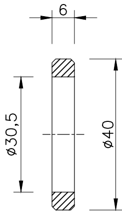
DISTANCE PIECE-01 NO
