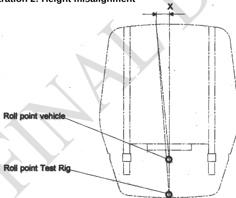
Illustration 2: Height misalignment –
