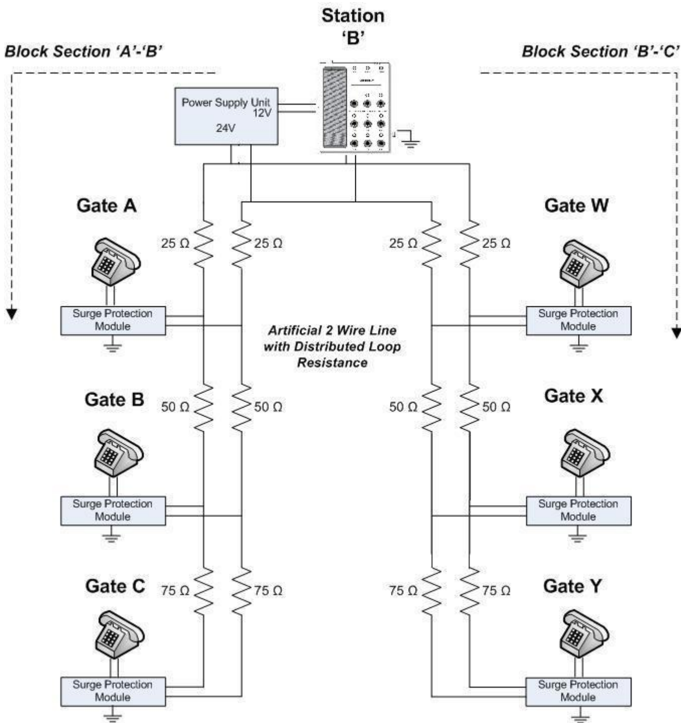
Figure-9 8: Test Setup for Performance Test of electronic LC Gate Telephone System with Station Telephone Unit and 6 Gate Telephones.
