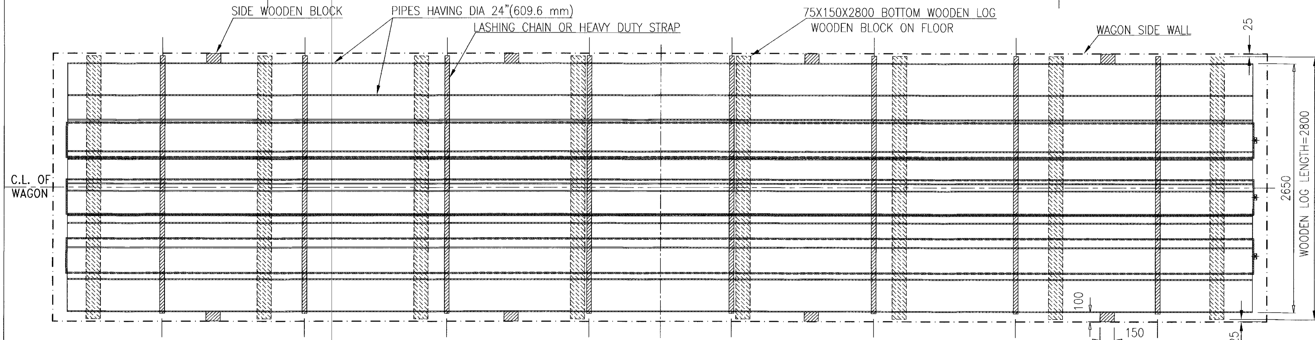
LOADING AND SECURING ARRANGEMENT DIAGRAM FOR 17 NOS OF 24" PIPES
