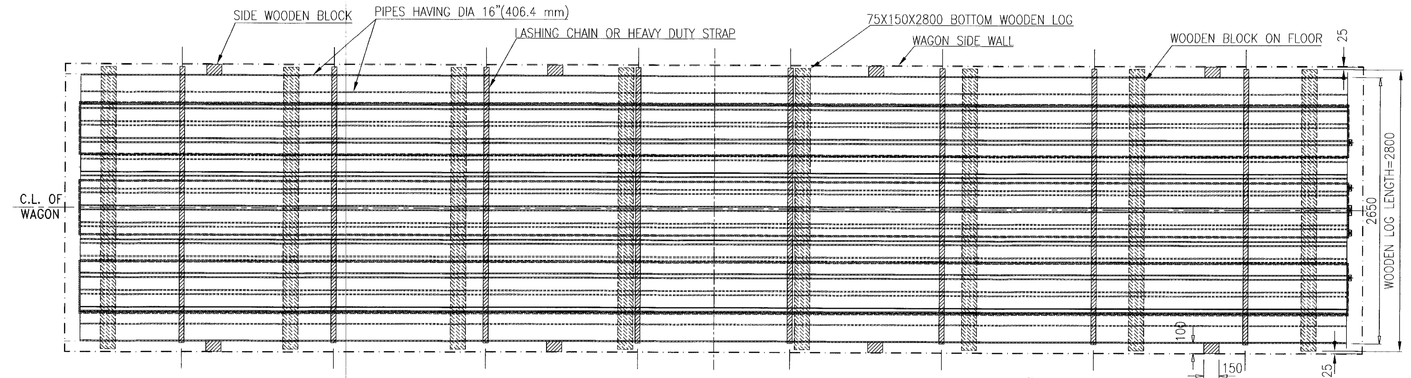
LOADING AND SECURING ARRANGEMENT DIAGRAM FOR 40 NOS OF 16" PIPES
