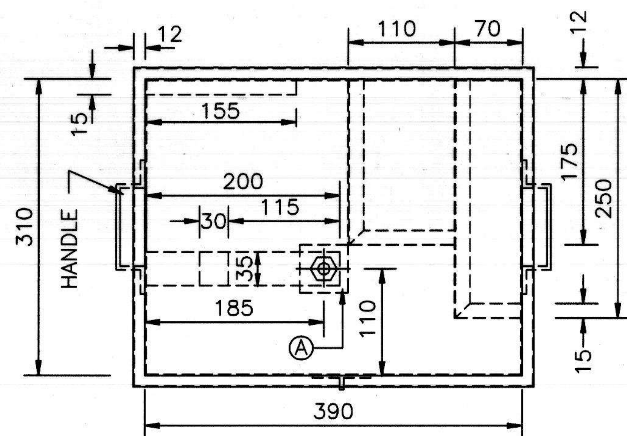
PLAN
