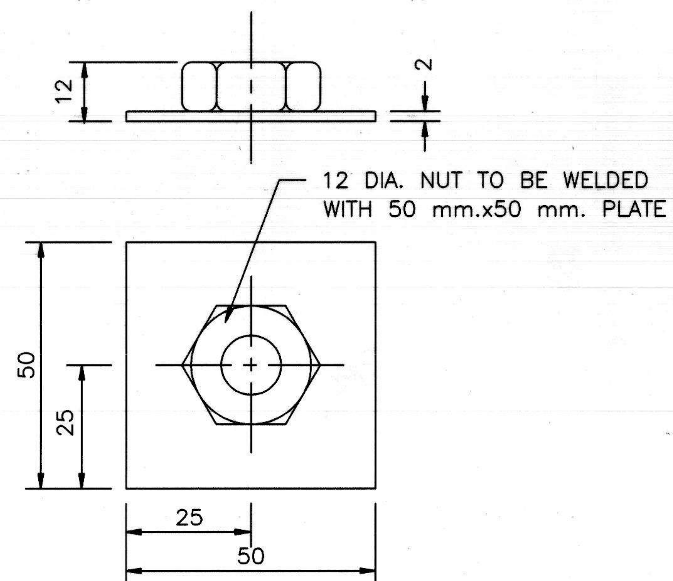
DETAILS AT 'A'
