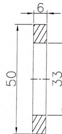
MACHINED WASHER-02Nos. WITH SPLIT PIN 6 X 60MM
