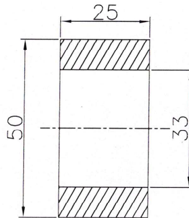
DISTANCE PIECE-02 Nos.
