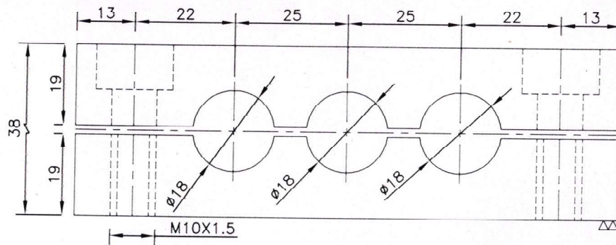
THREE HOSE
