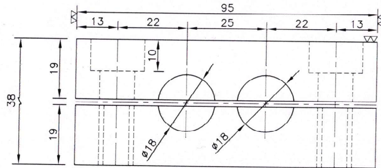
TWO HOSE
