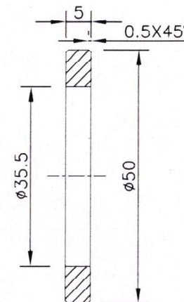
MACHINED WASHER-02 NO WITH SPLIT PIN 8X60MM-02 NO
