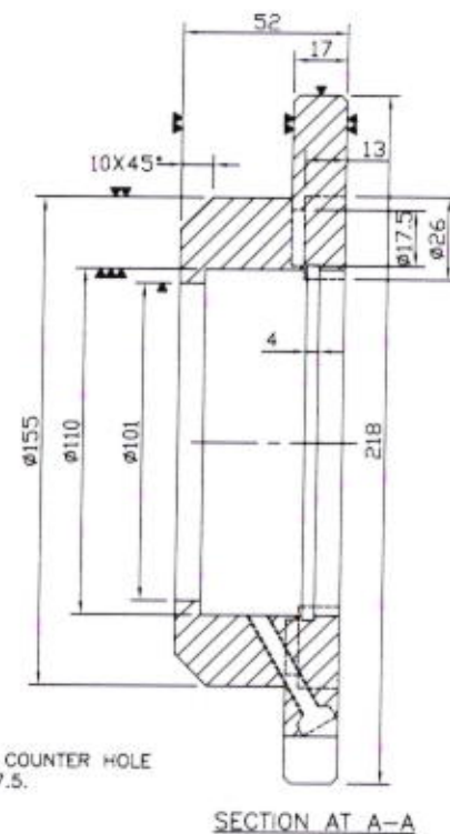
SECTION AT A-A
