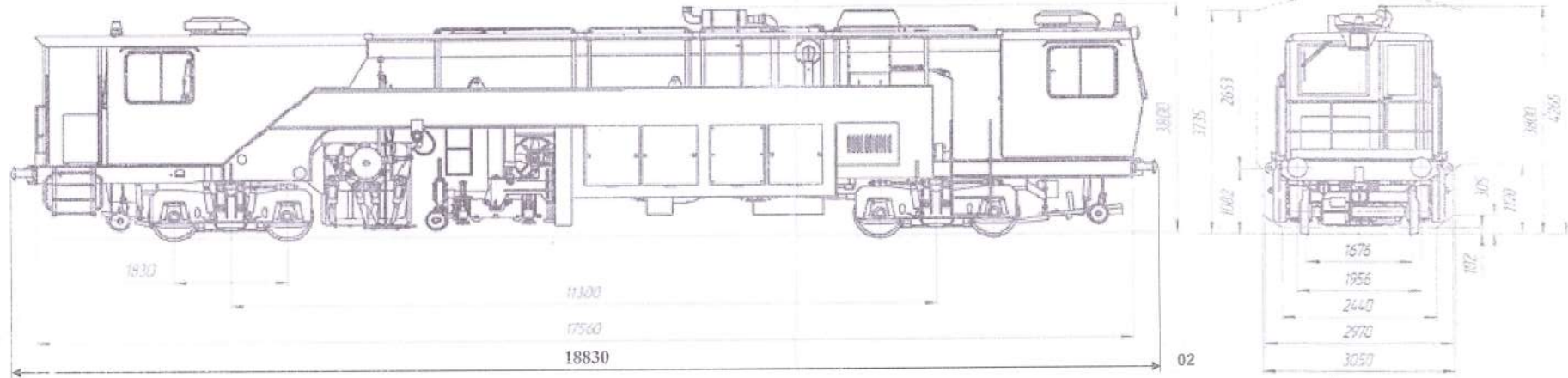
1 (ALTM) PMA-1M Worksite Tamper, general view, principal data and dimensions (mm)
