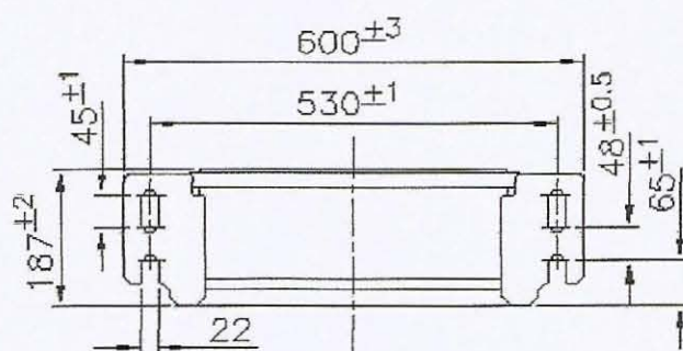
SUPPORTING DEVICE
