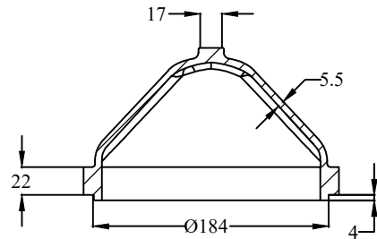
SECTION B-B SCALE 1 : 3.5
