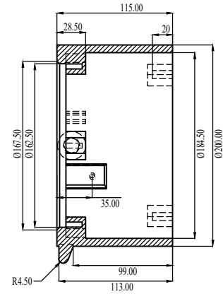
SECTION E-E
