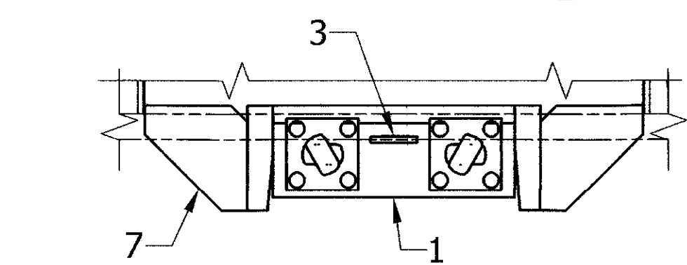
DETAIL C FOR WELDING AND DETAILS REFER DETAIL-C IN WD-22062-S-23
