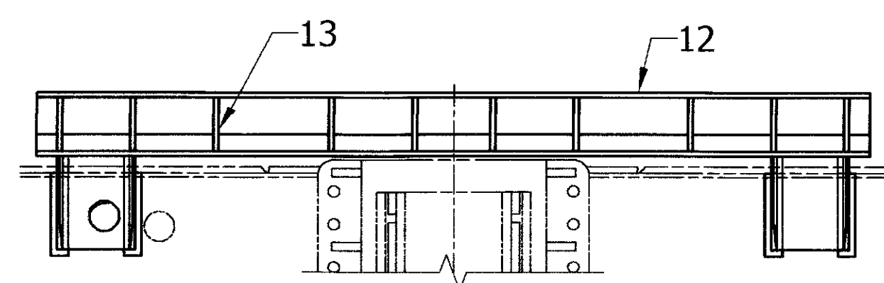
B-END APD ARRANGEMENT FOR DETAILS REFER DWG WD-22062-S-23
