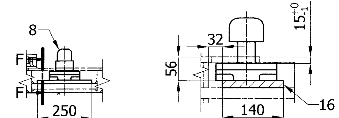
SECTION F-F
