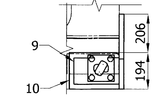
DETAIL A FOR WELDING AND DETAILS REFER DETAIL-A IN WD-22062-S-23
