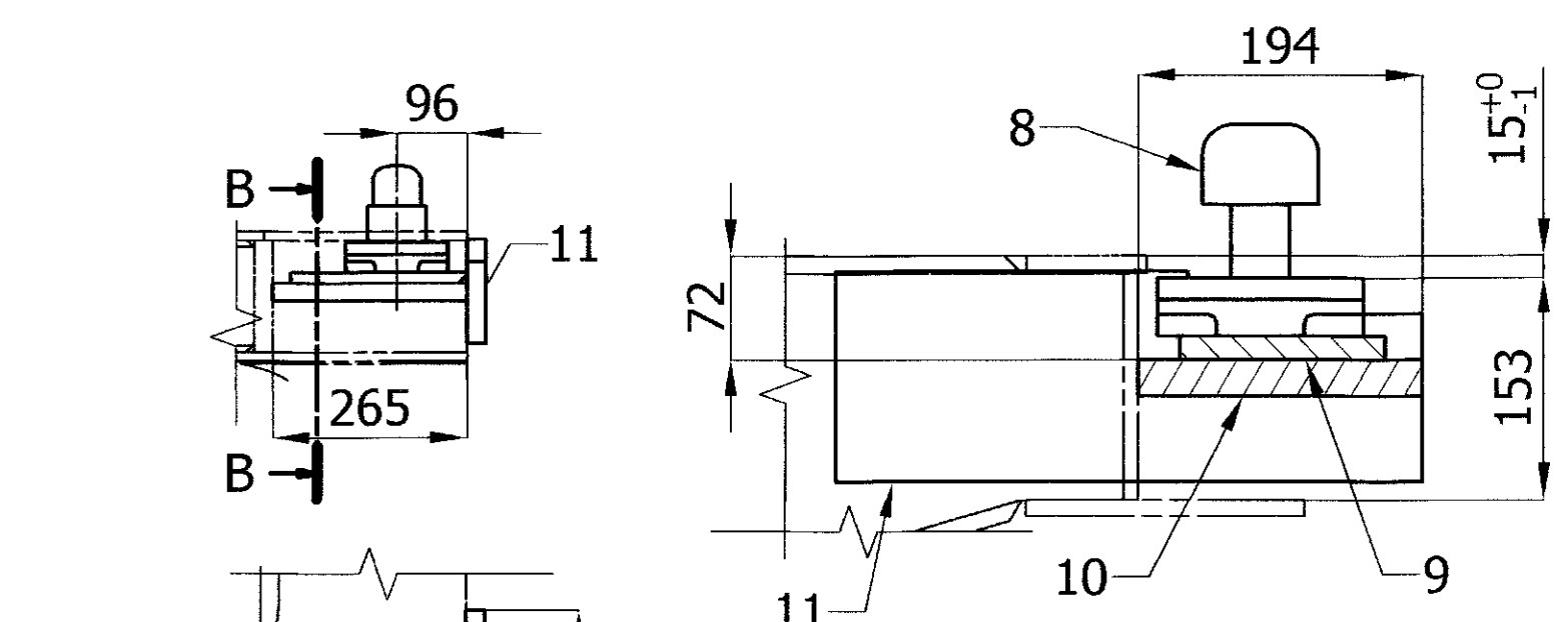
SECTION B-B
