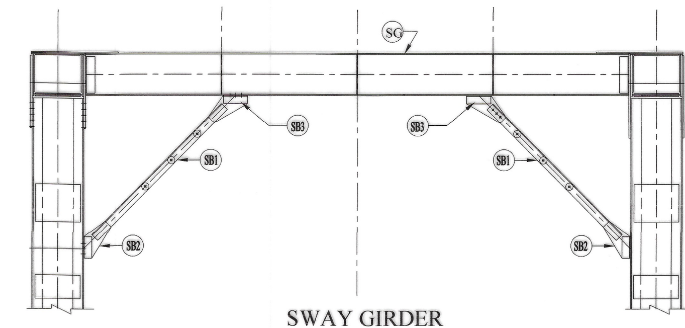
SWAY GIRDER
