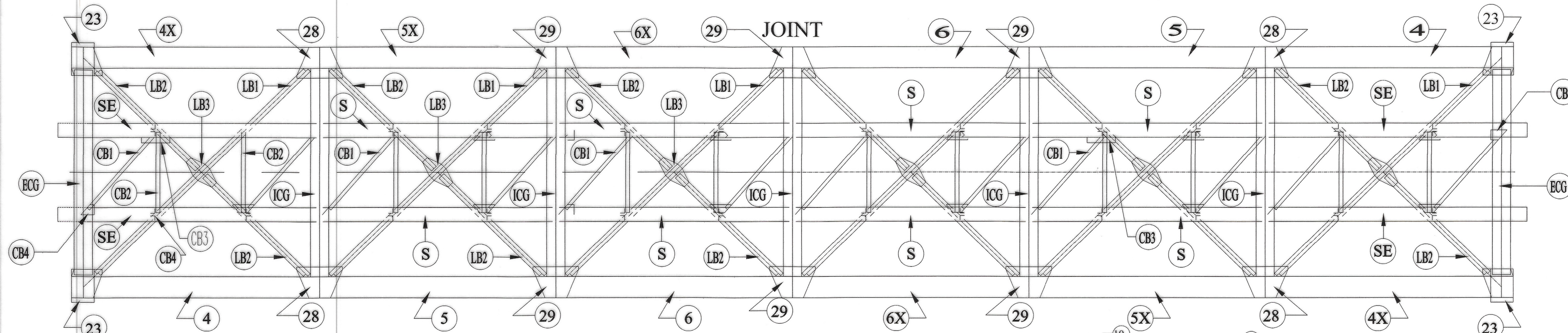
BOTTOM PLAN
